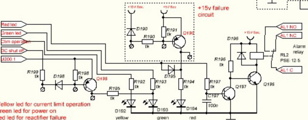
Schematic drawing for 11826.BV3 Monitoring and alarm circuits A/S ELTEK
